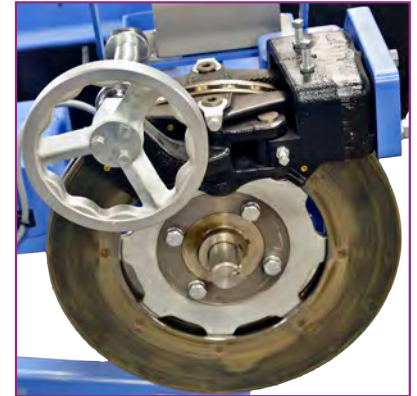
16" Bronze Ventilated Mechanical Disc Tension Brake
