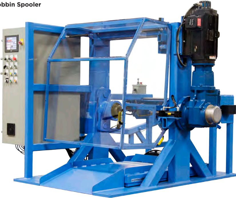
ILWT2.5 2,500lb Bobbin Spooler
