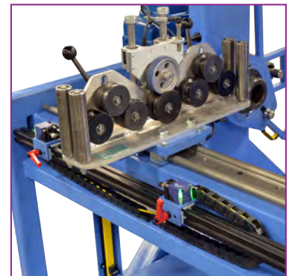
High Speed Measurer Semi-Straightener
