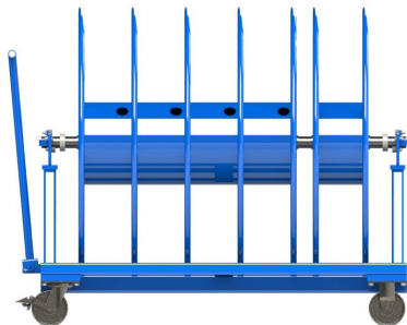
One 1-position freespinning reel & one 4-position reel
