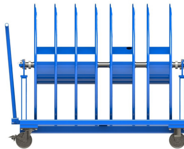
Two 1-position freespinning reels & one 3-position reel
