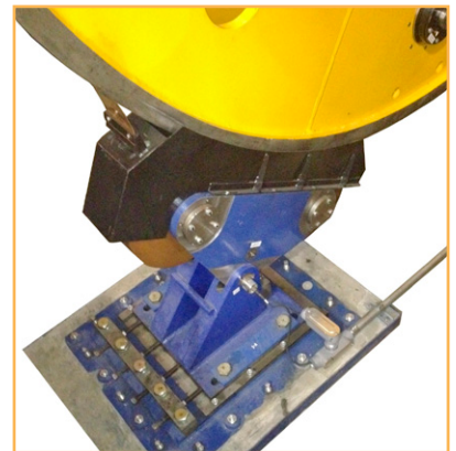
Floor Mounts with Brake
