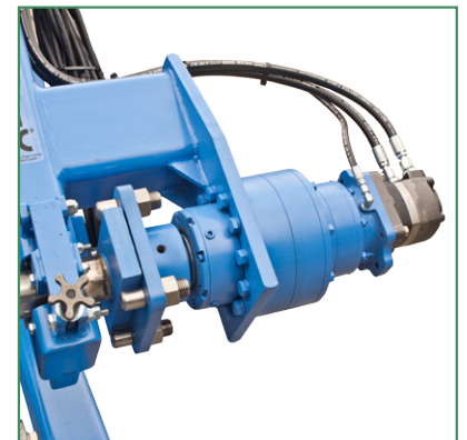
"Drop -in" Reel Shaft with Direct Hydraulic Drive
