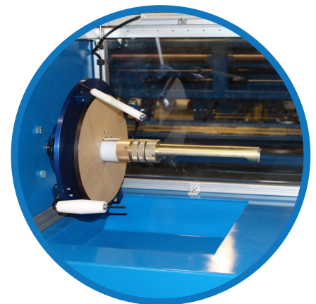
TAPING HEAD
