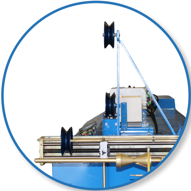
Automatic Levelwind with V-Groove Guide Sheaves
